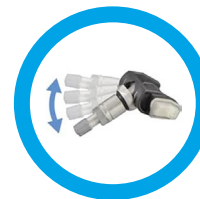
Adjustable Angle Aluminum Clamp-In Part #33700
